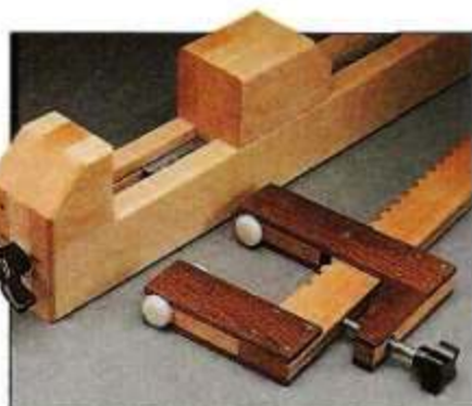
Shop-Built Clamps page 12
