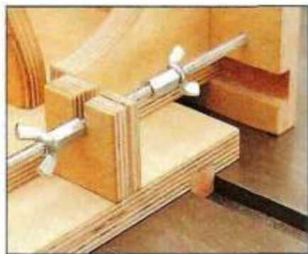
Tenoning Jig page 16
