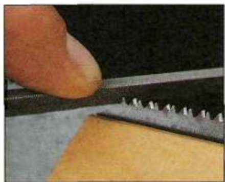
▲ Filing: A triangular file is then used to sharpen the teeth of the saw once they've been jointed and set.
