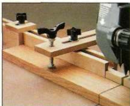
Radial Arm Saw Fence page 7
