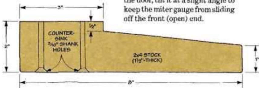
▲ A quick-access holder is mounted to the cabinet for your miter gauge. It allows you to slide the miter gauge in place — even with an auxiliary fence attached.
